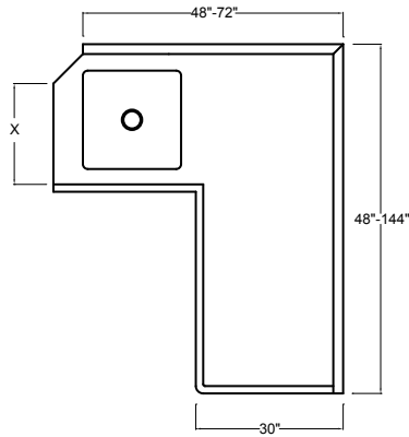
L Shape Corner
