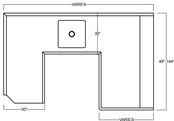
U Shape Landing
