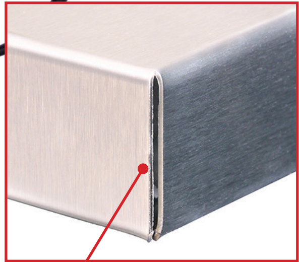
Typical non-welded corner design
