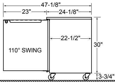
SIDE VIEW 20" DOOR OPENING
