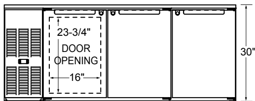
FRONT VIEW 16" DOOR OPENING
