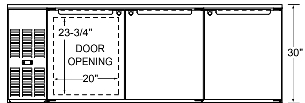
FRONT VIEW 20" DOOR OPENING
