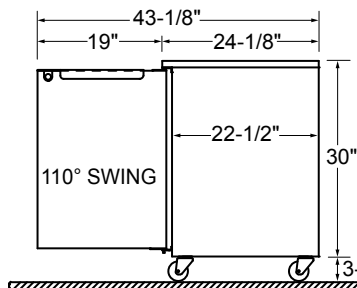
SIDE VIEW 16" DOOR OPENING
