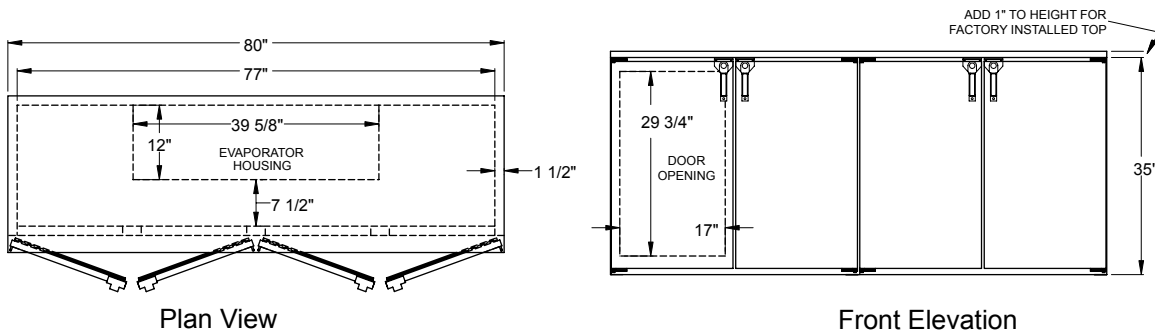
Plan View
