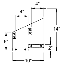
SIDE ELEVATION
