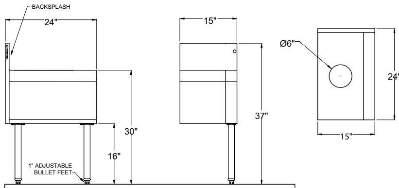
SIDE ELEVATION
