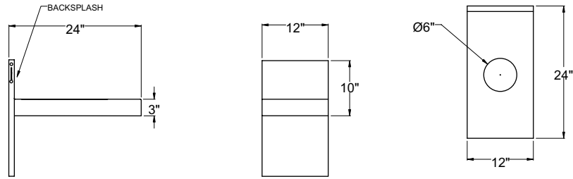
SIDE ELEVATION
